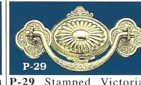
P-29 Stamped Victorian Eastlake brass handle set. Boring at 3"; overall size: 1 7/8" tall by 4 1/8" wide--cast posts (can use panhead screws from the back.)
