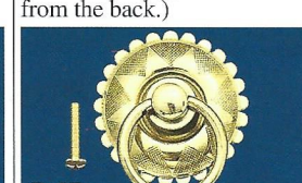
D-1B Large backplate ring pull for larger drawers or to cover damaged wood. Ring is 1 3/4" dia. and the backplate is 2 9/16" diameter. Thickness of D-1A & D-1B wrought backplate: 3/64" (1mm). D-1A & D-1B use 8/32 thread
