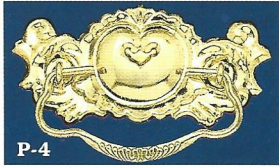
P-4 Stamped "heart motif" Victorian brass handle set with a boring of 3". Overall size: 2 3/8" x 4 7/8".
